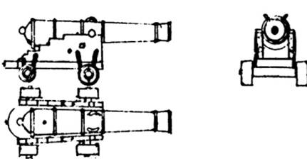
Iron 8-pounder (8)
