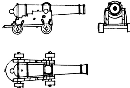
Iron 12 pounder (4)
