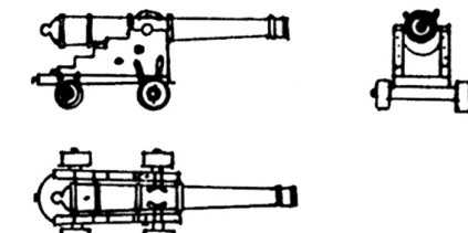
Metal 6-pounder (drake) (2)
