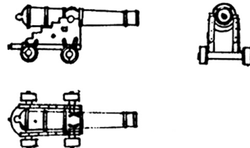
Iron 4-pounder (4)
