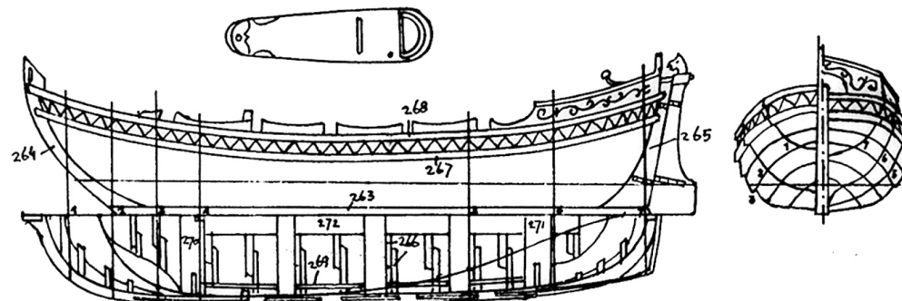
Shallop, long between stem and stern 26 feet, wide 7 feet
